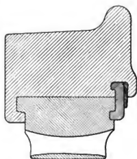
Fig. 4560. Carleton- Stroudlley Fastening.
